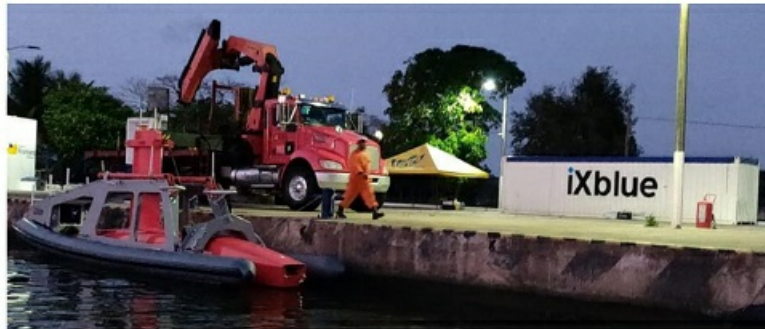
Full DriX package in operation
