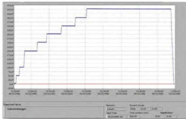
Image 38: Example test of a 4000m housing with 450 Bar test pressure.
